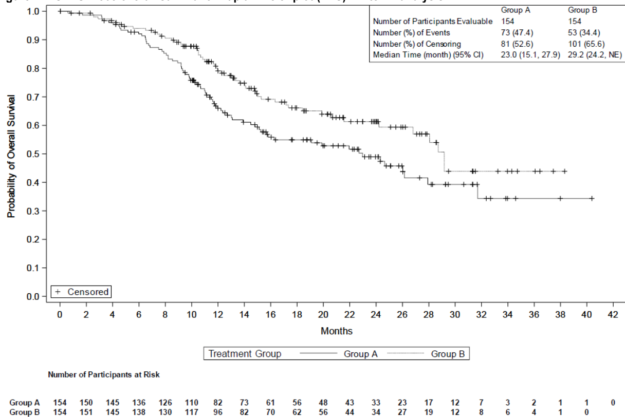
Figure 2: POD1UM-303 overall survival of Kaplan-Meier plot (FAS) – interim analysis
