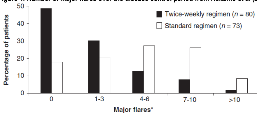
Figure 4: Number of major flares over the disease control period from Reitamo et al (2010)
